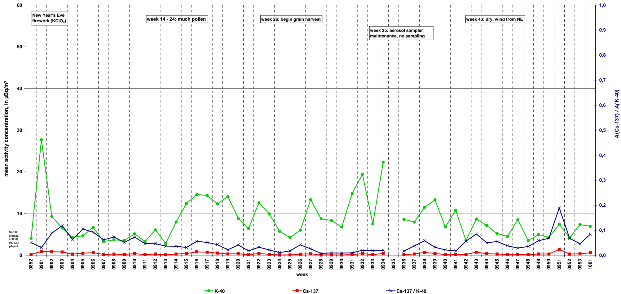
K-40 and Cs-137 in ground-level air in Braunschweig 2009
