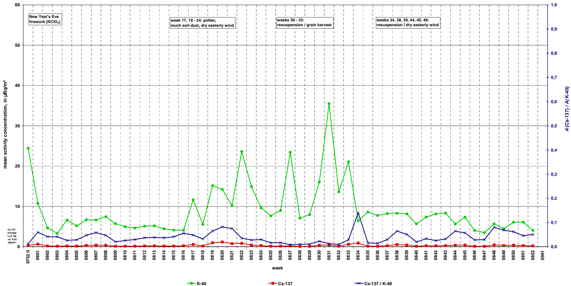
K-40 and Cs-137 in ground-level air in Braunschweig 2008
