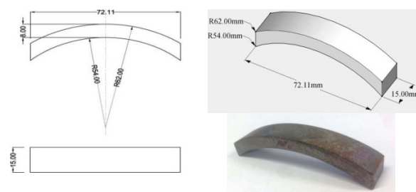
Fig. 1 Curved magnet with dimensions
