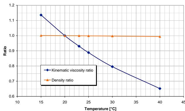
Fig. 2 Ratios of kinematic viscosity and density of water vs. temperature (according to [6] and [7], respectively)
