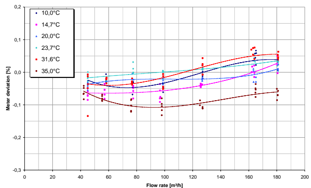
Fig.10 Error curves of a DN100 Coriolis flowmeter: Temperature: 10°C ... 35°C
