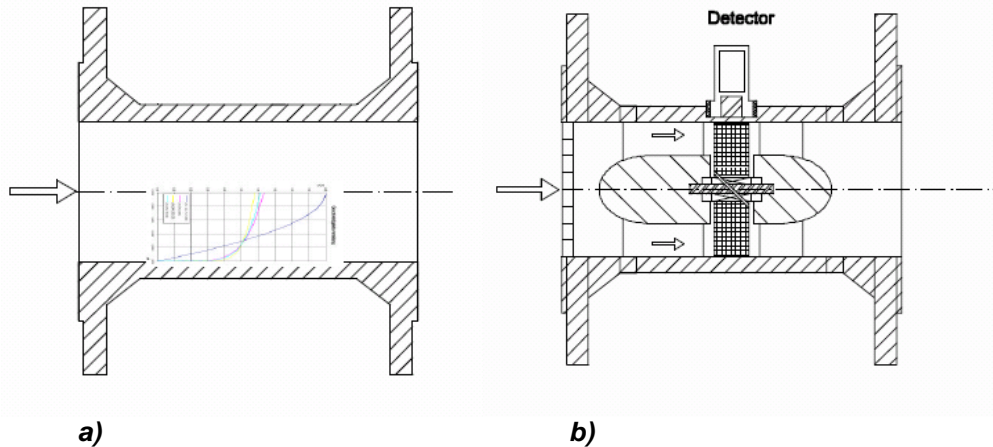
Fig. 1 Flow conditions in a straight pipe and a pipe with inserted flow sensor a) Flow velocity profile in straight pipe b) Pipe with turbine as sensor sensing element
