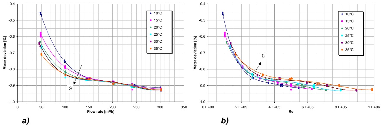
Fig. 7 Error curves of a DN150 turbine flowmeter: temperature correction applying Equ. (4) a) Meter error vs. flow rate b) Meter error vs. Re number
