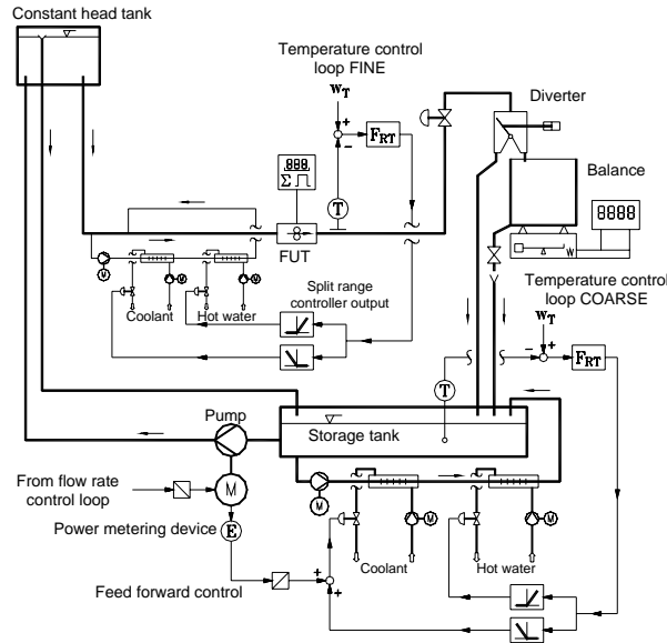
Fig. 4 Temperature control loops
