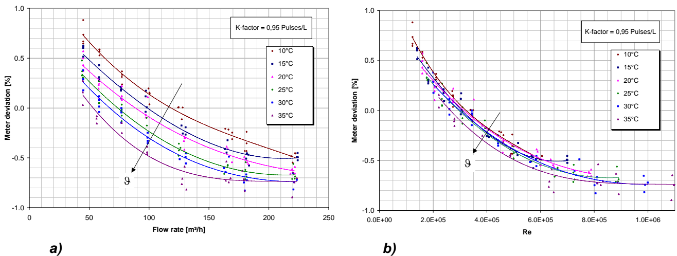
Fig. 8 Error curves of a DN100 vortex-shedding flowmeter: “raw” signal a) Meter error vs. flow rate b) Meter error vs. Re number
