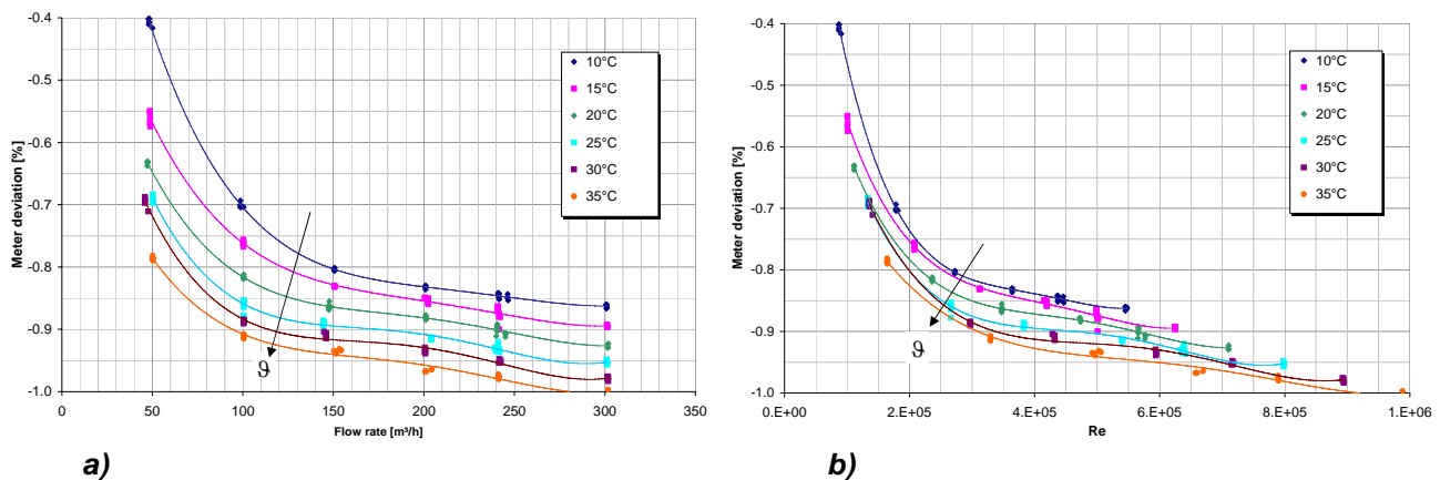
Fig. 6 Error curves of a DN150 turbine flowmeter: “raw” data
